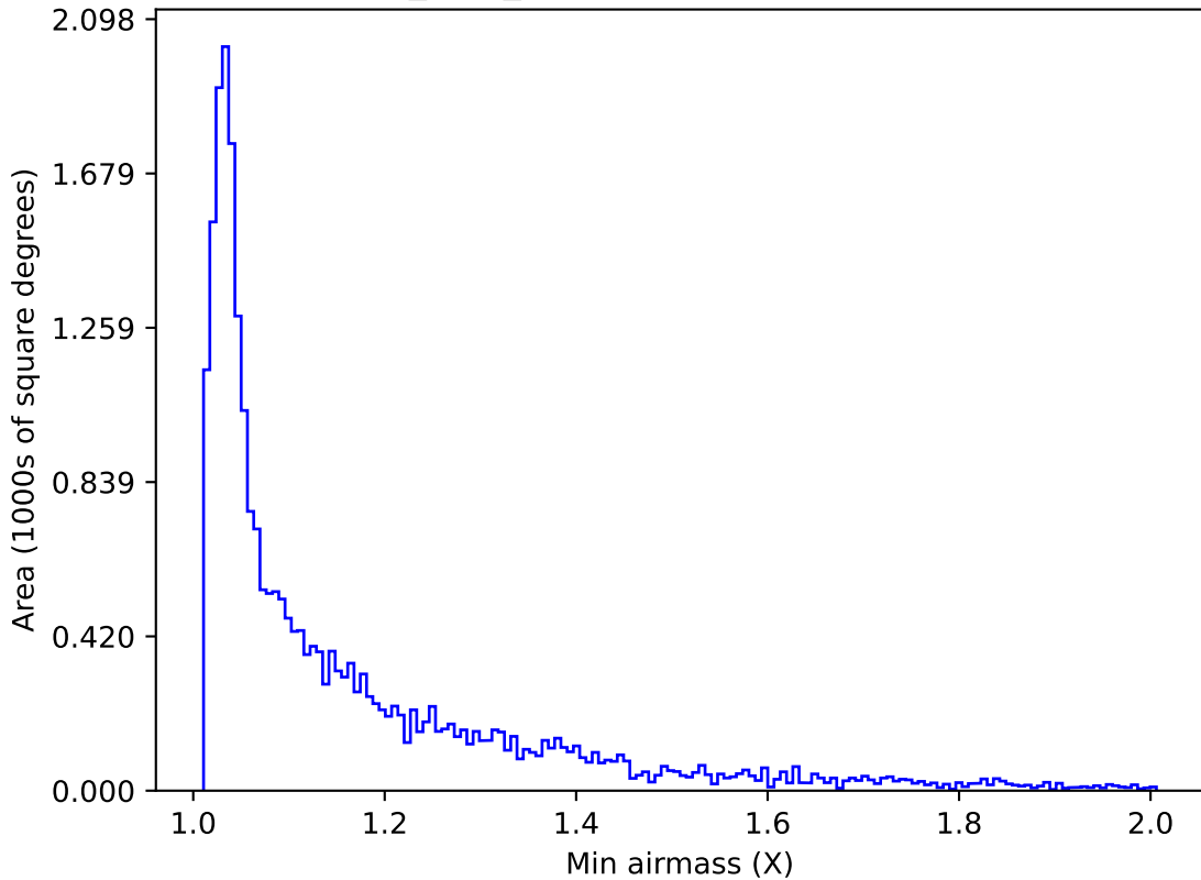
roman_v3.3_10yrs Yr 1 z band: Min airmass
