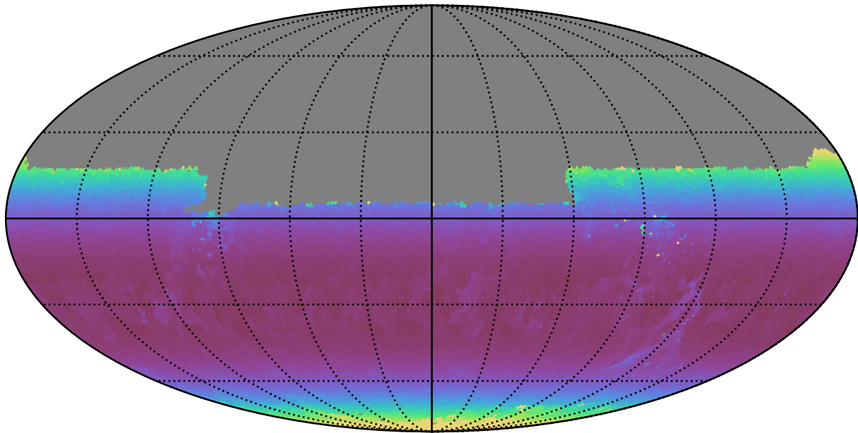
roman_v3.3_10yrs Yr 1 y band: Min airmass
