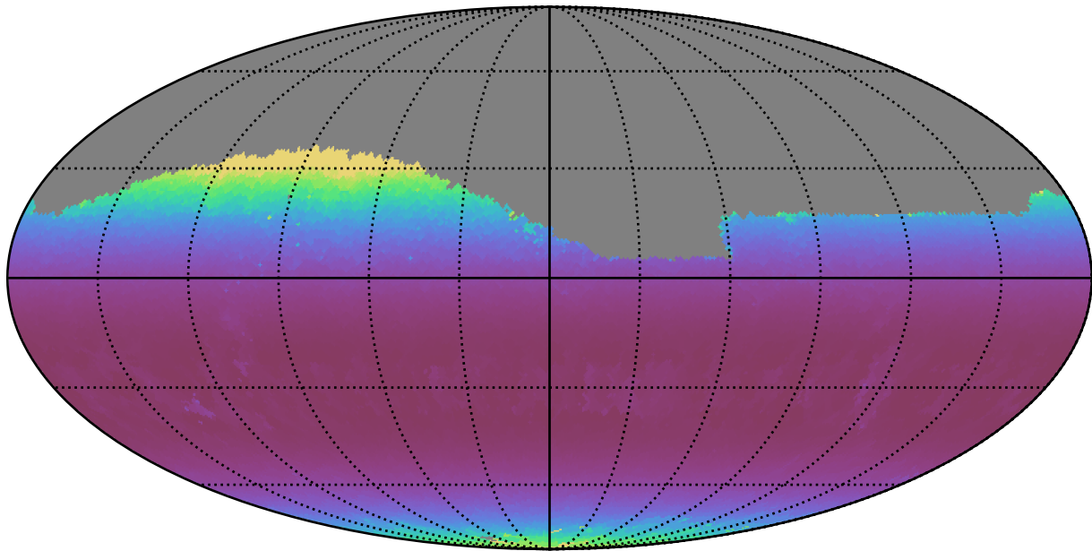
roman_v3.3_10yrs Yr 1 r band: Min airmass
