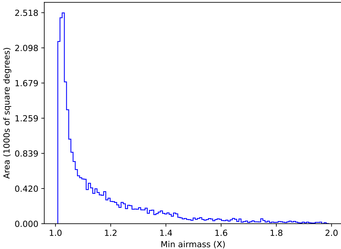
roman_v3.3_10yrs Yr 1 i band: Min airmass
