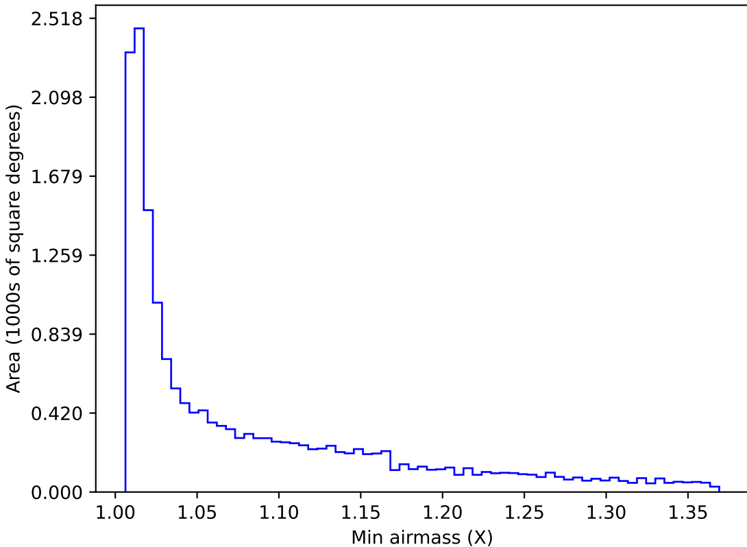
roman_v3.3_10yrs WFD z band: Min airmass
