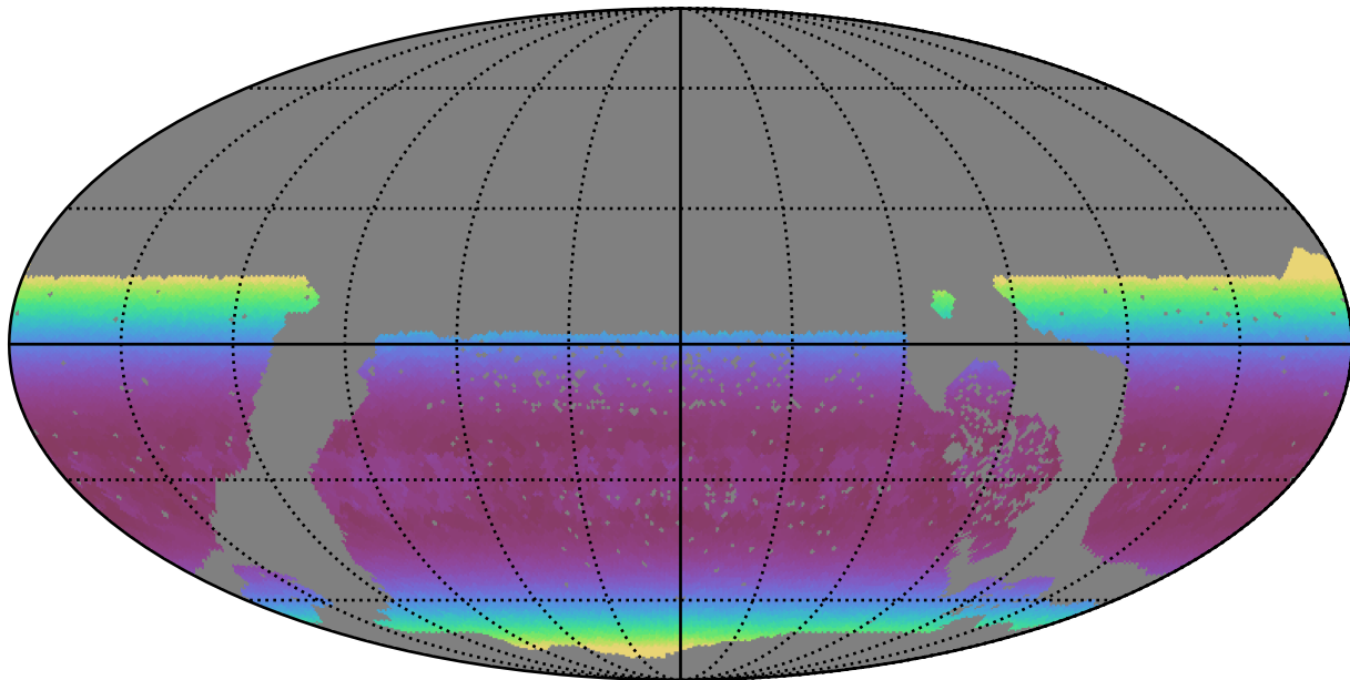
roman_v3.3_10yrs WFD u band: Min airmass
