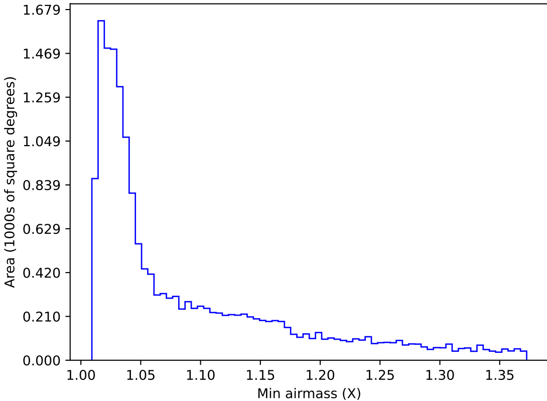
roman_v3.3_10yrs WFD u band: Min airmass
