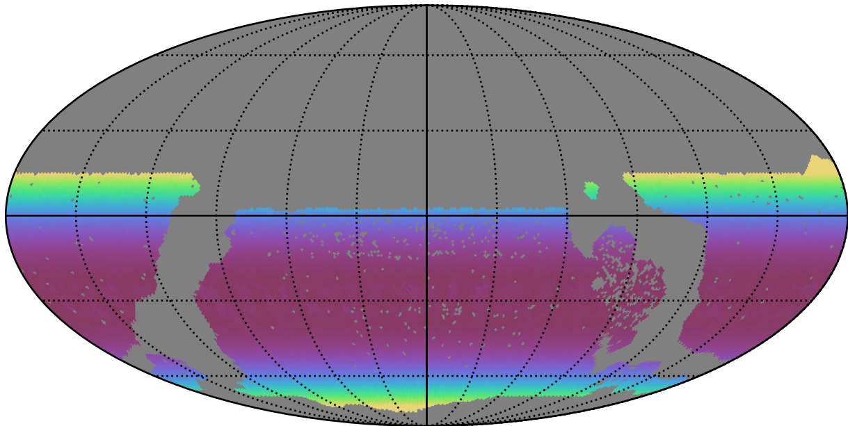
roman_v3.3_10yrs WFD i band: Min airmass
