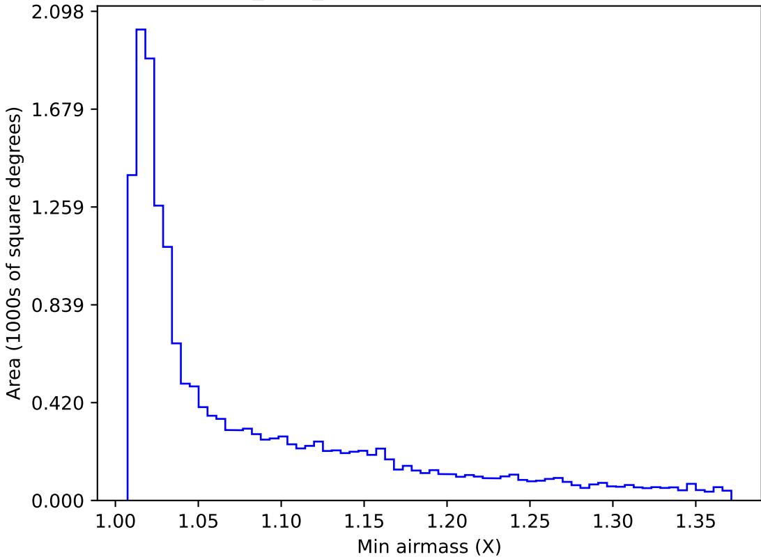
roman_v3.3_10yrs WFD g band: Min airmass
