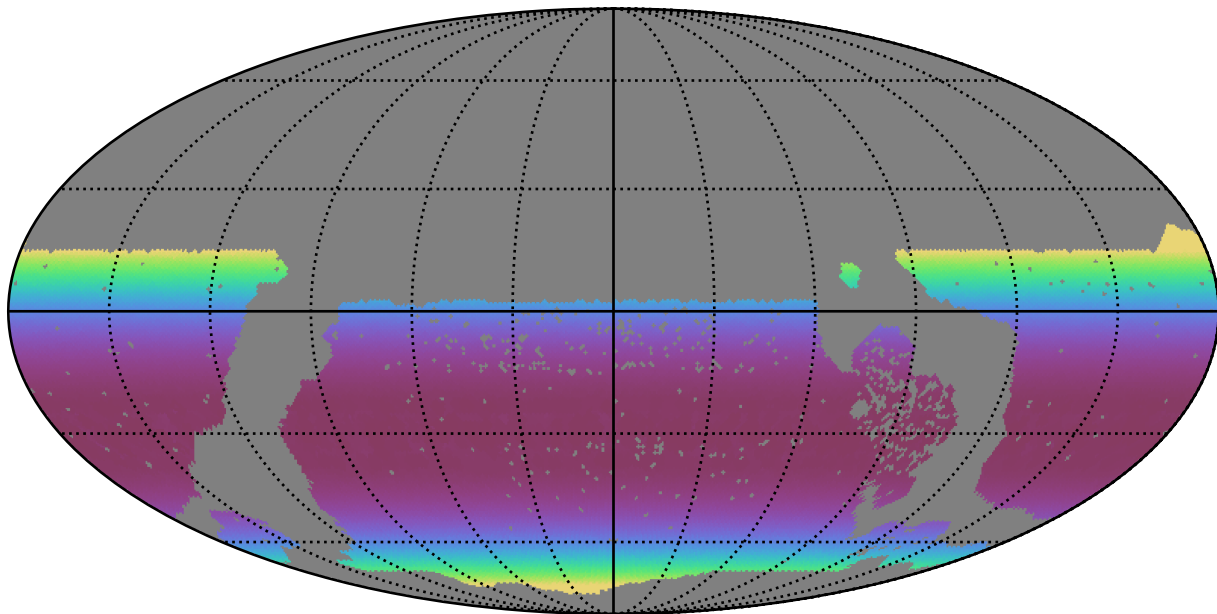
roman_v3.3_10yrs WFD all bands: Min airmass
