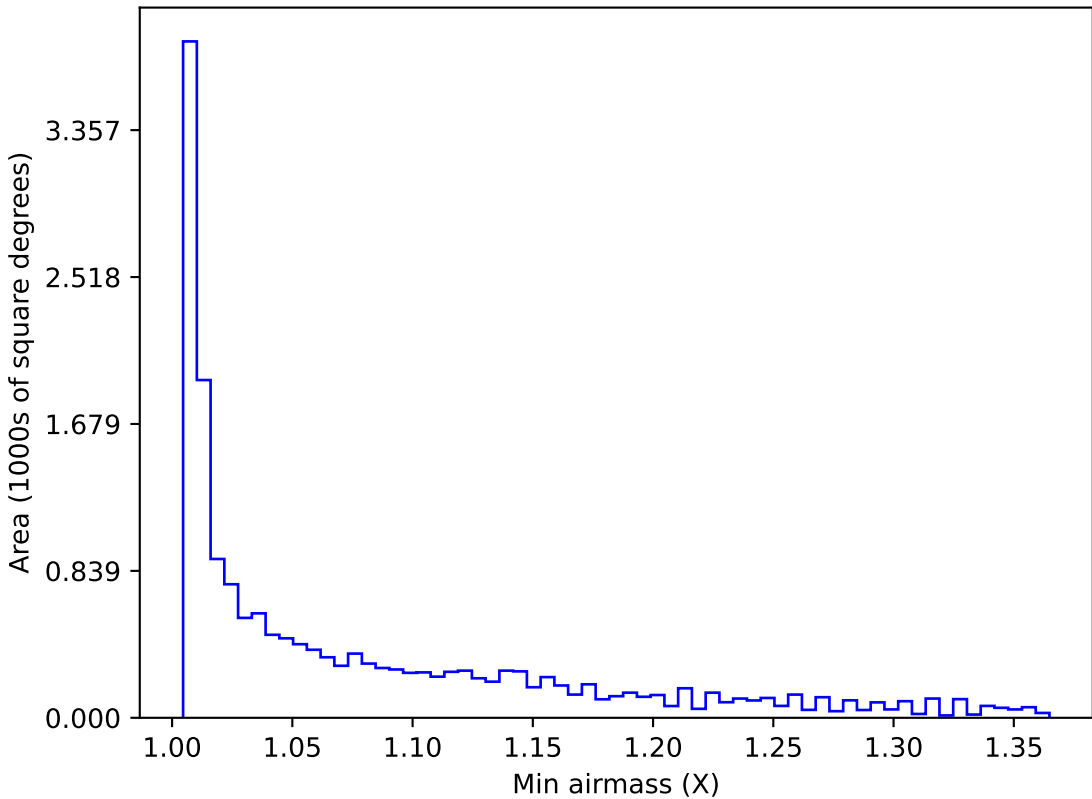
roman_v3.3_10yrs WFD all bands: Min airmass
