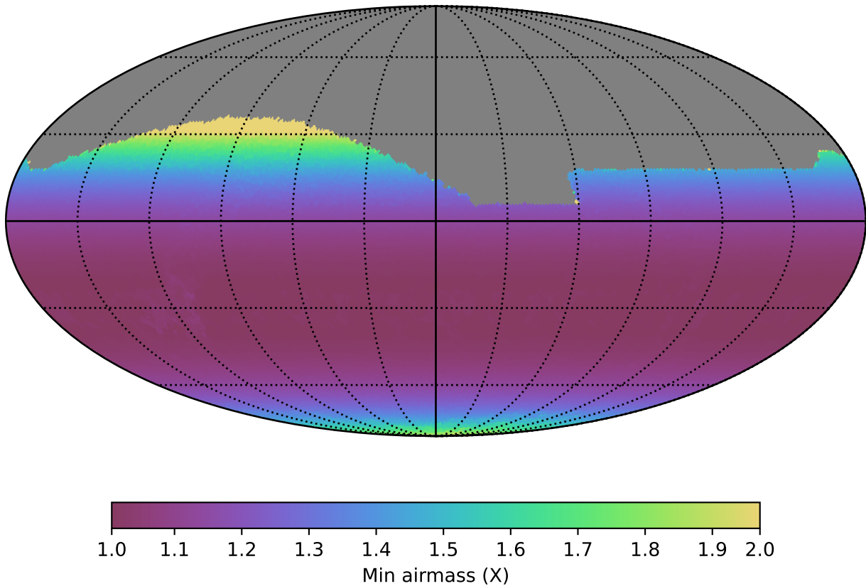
roman_v3.3_10yrs All sky z band: Min airmass
