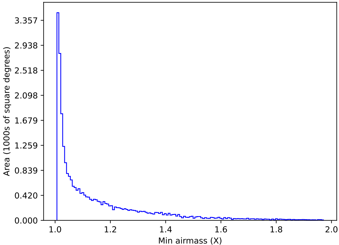
roman_v3.3_10yrs All sky z band: Min airmass
