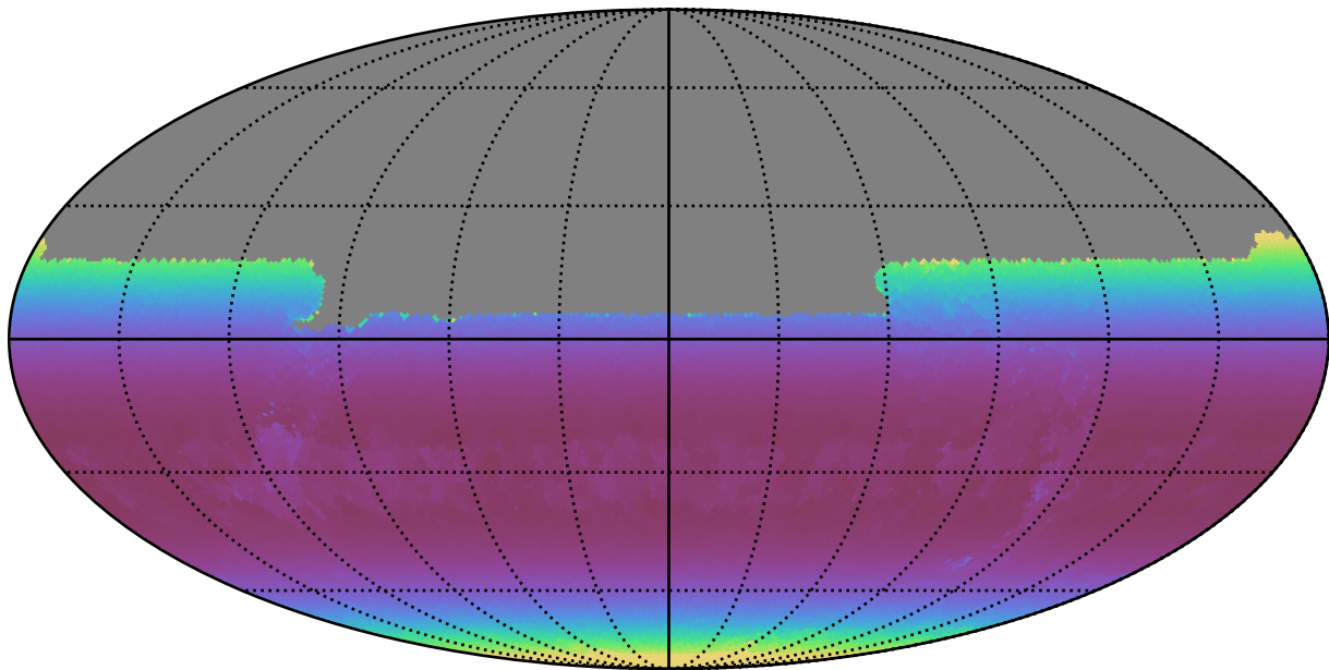
roman_v3.3_10yrs All sky u band: Min airmass
