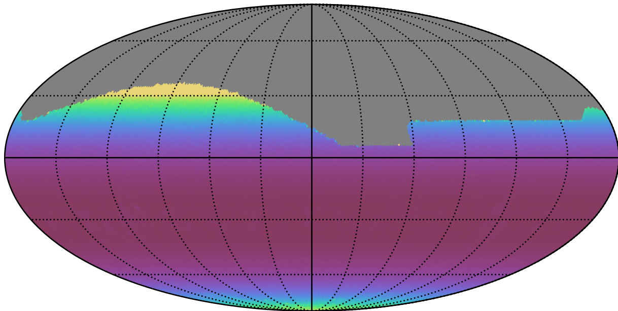
roman_v3.3_10yrs All sky r band: Min airmass
