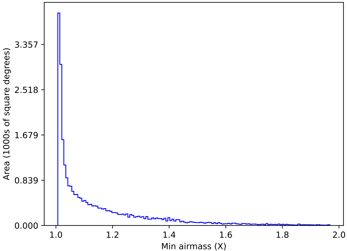
roman_v3.3_10yrs All sky r band: Min airmass
