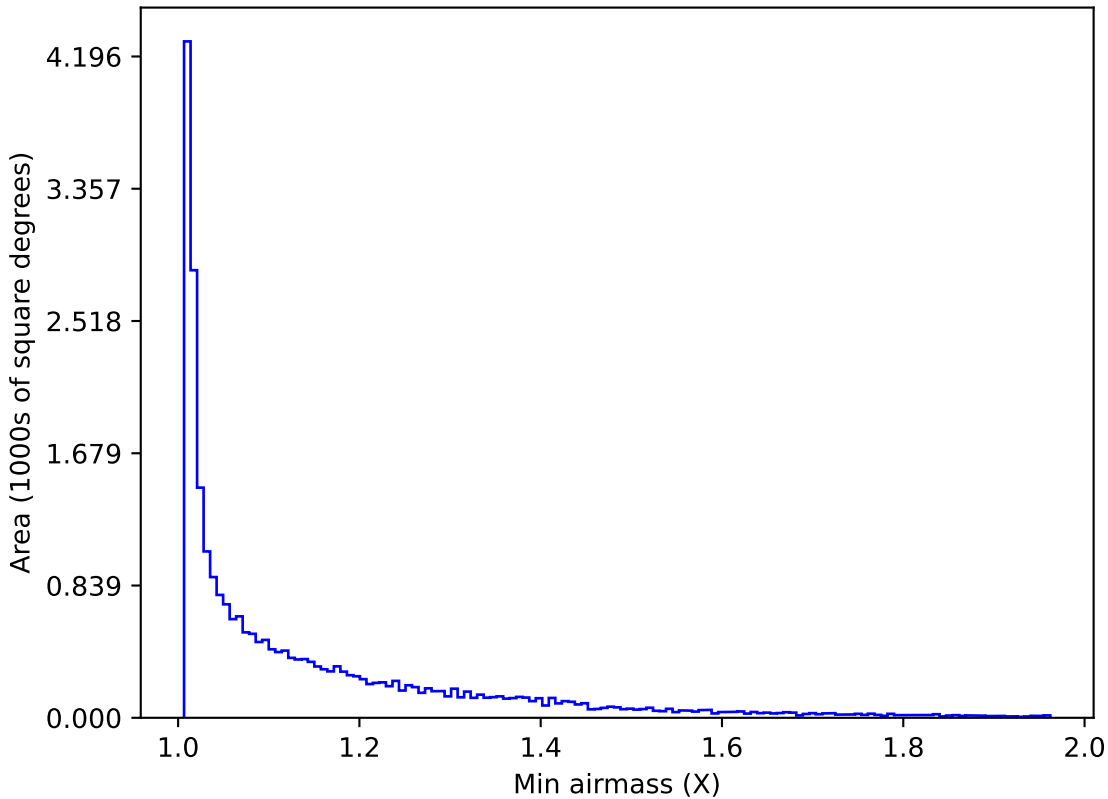
roman_v3.3_10yrs All sky i band: Min airmass
