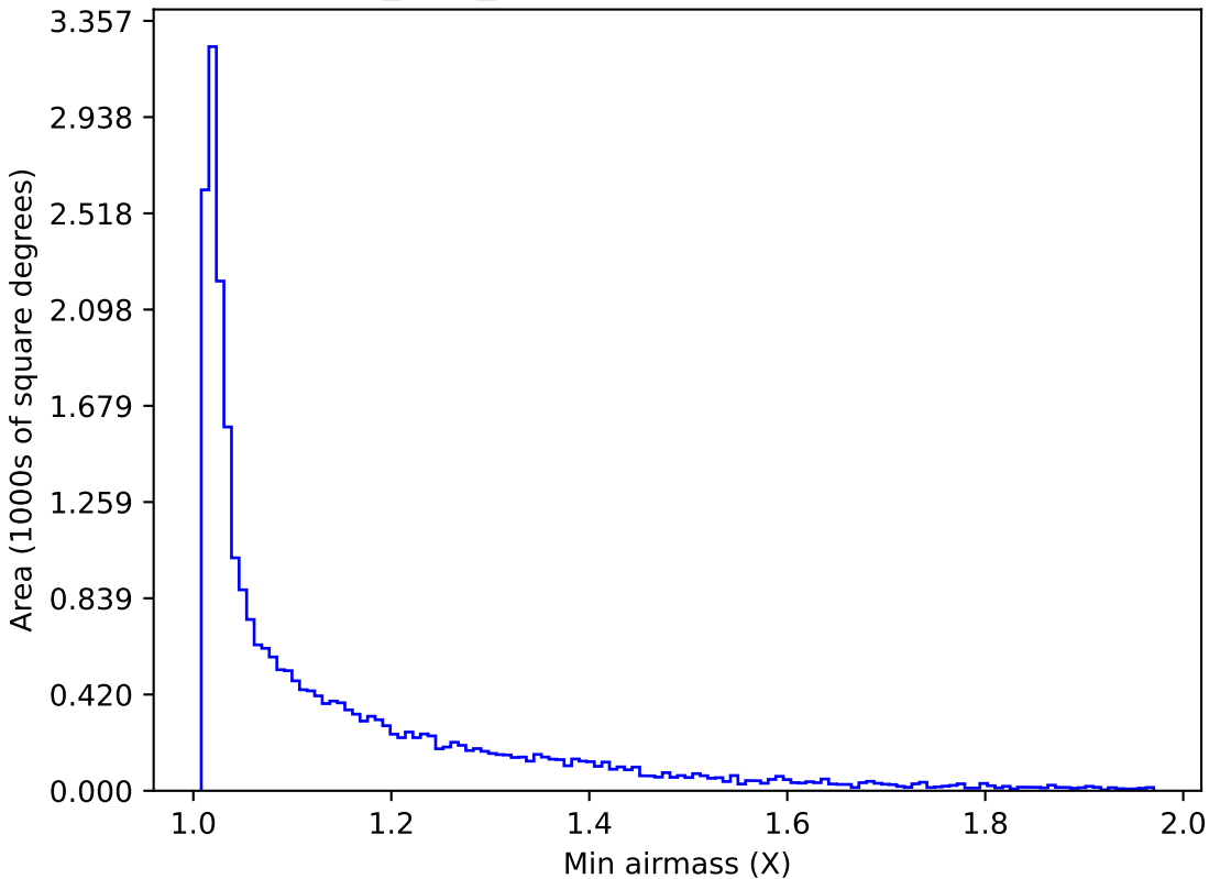
roman_v3.3_10yrs All sky g band: Min airmass
