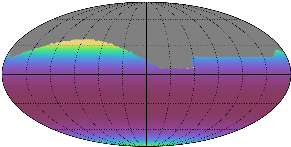
roman_v3.3_10yrs All sky all bands: Min airmass
