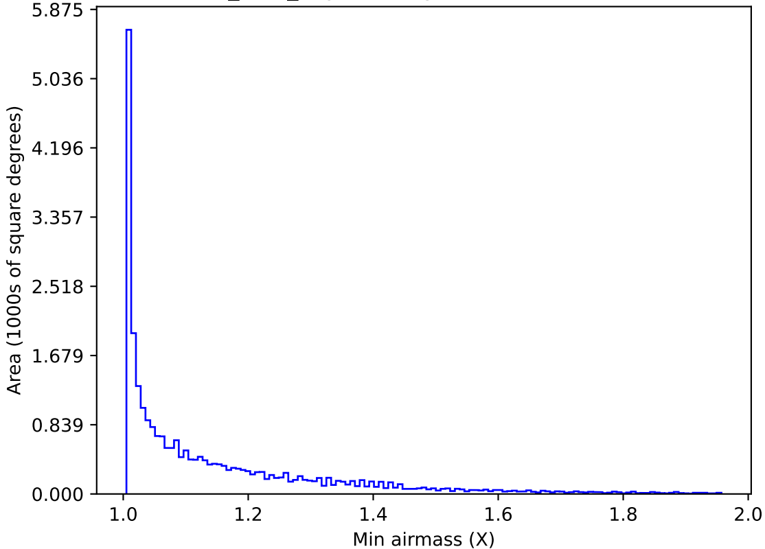
roman_v3.3_10yrs All sky all bands: Min airmass
