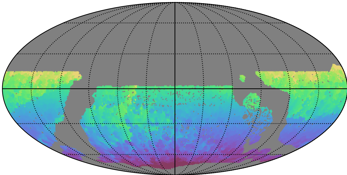
roman_v3.3_10yrs WFD all bands: Min HA
