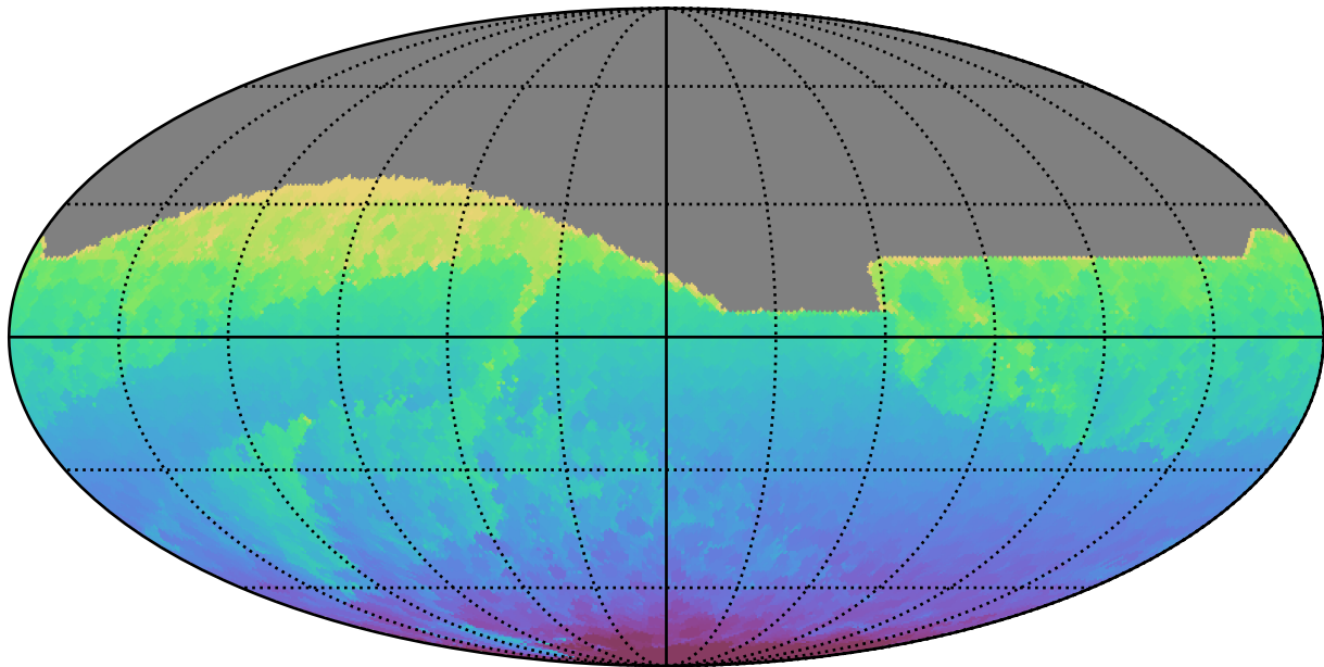
roman_v3.3_10yrs All sky all bands: Min HA
