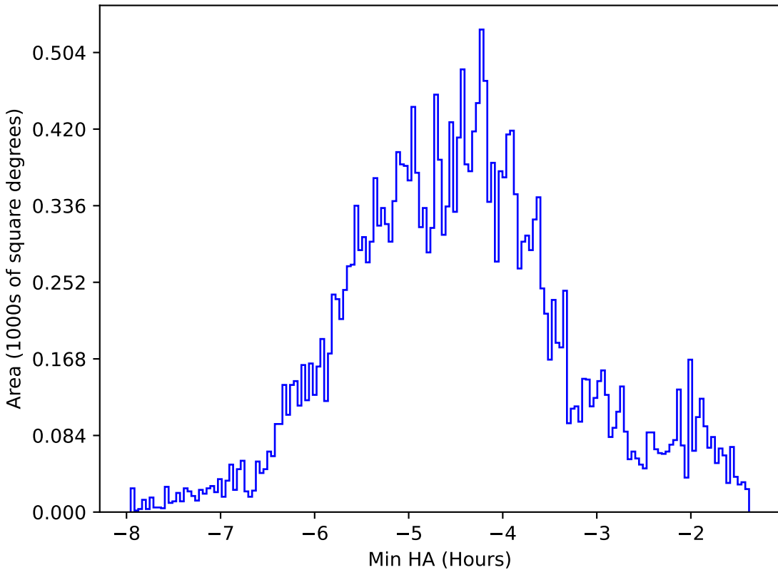
roman_v3.3_10yrs All sky all bands: Min HA
