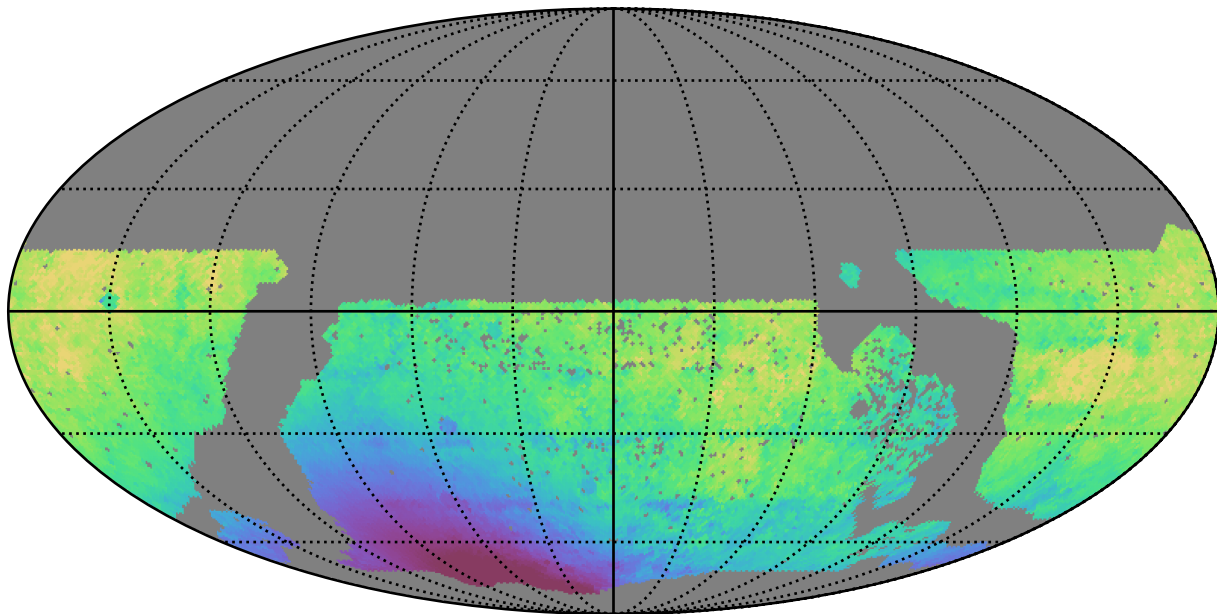
roman_v3.3_10yrs WFD z band: Median solarElong
