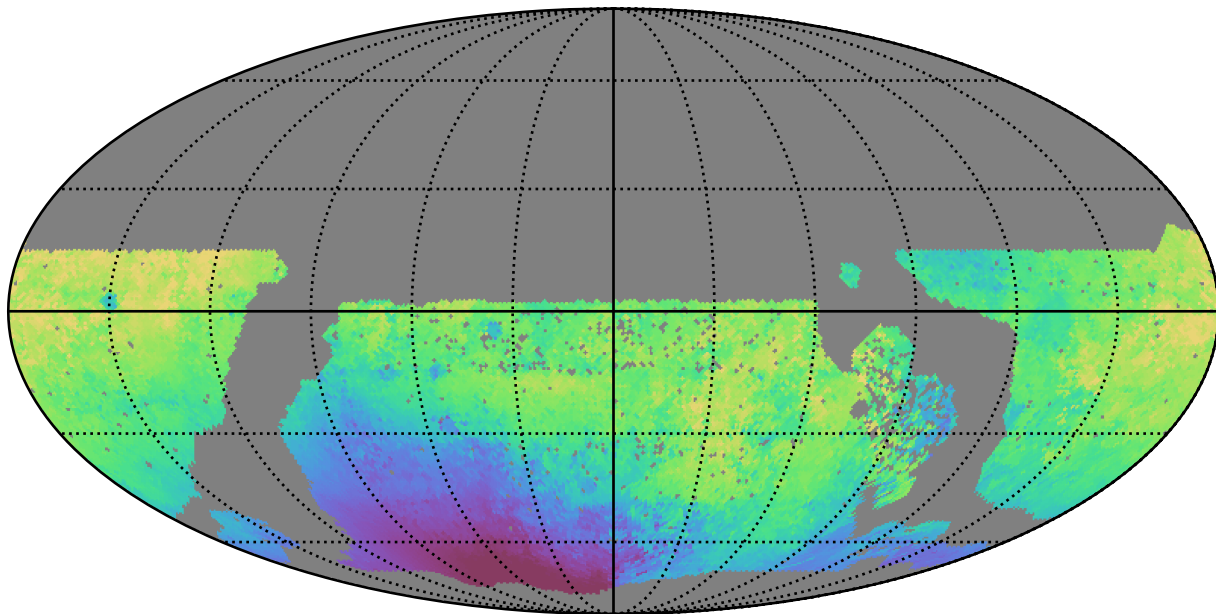
roman_v3.3_10yrs WFD u band: Median solarElong
