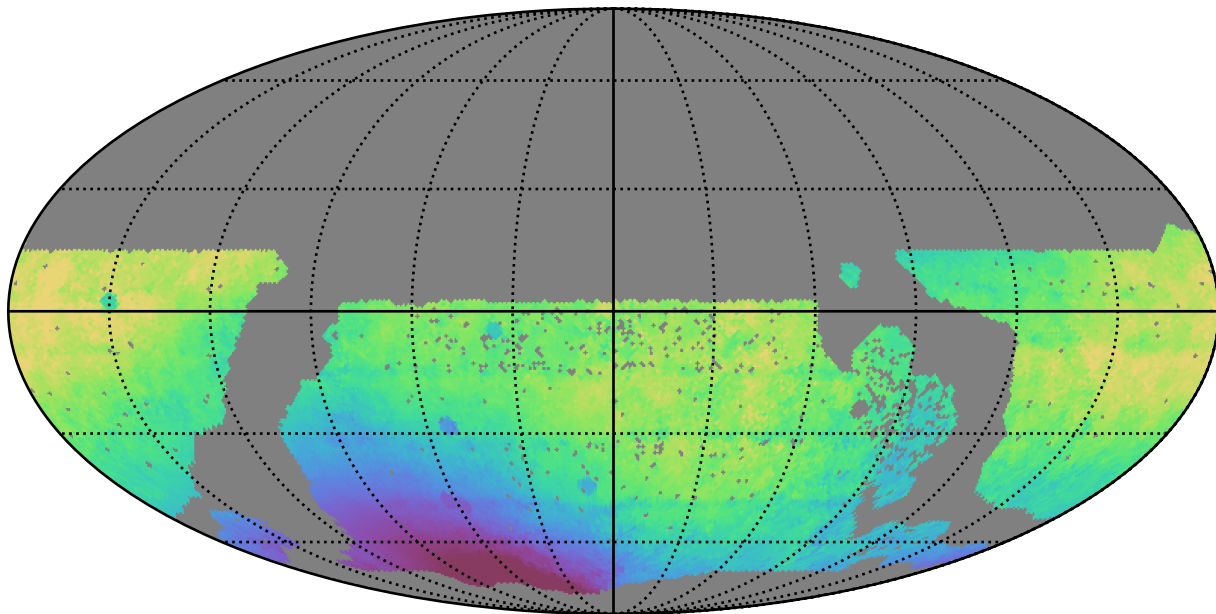
roman_v3.3_10yrs WFD r band: Median solarElong
