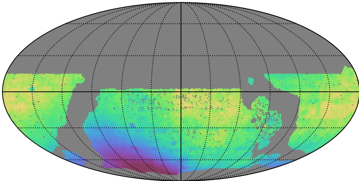
roman_v3.3_10yrs WFD i band: Median solarElong
