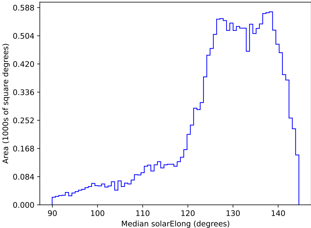
roman_v3.3_10yrs WFD i band: Median solarElong
