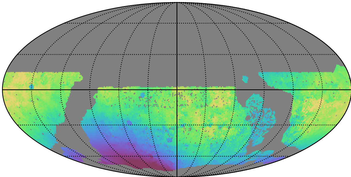
roman_v3.3_10yrs WFD g band: Median solarElong
