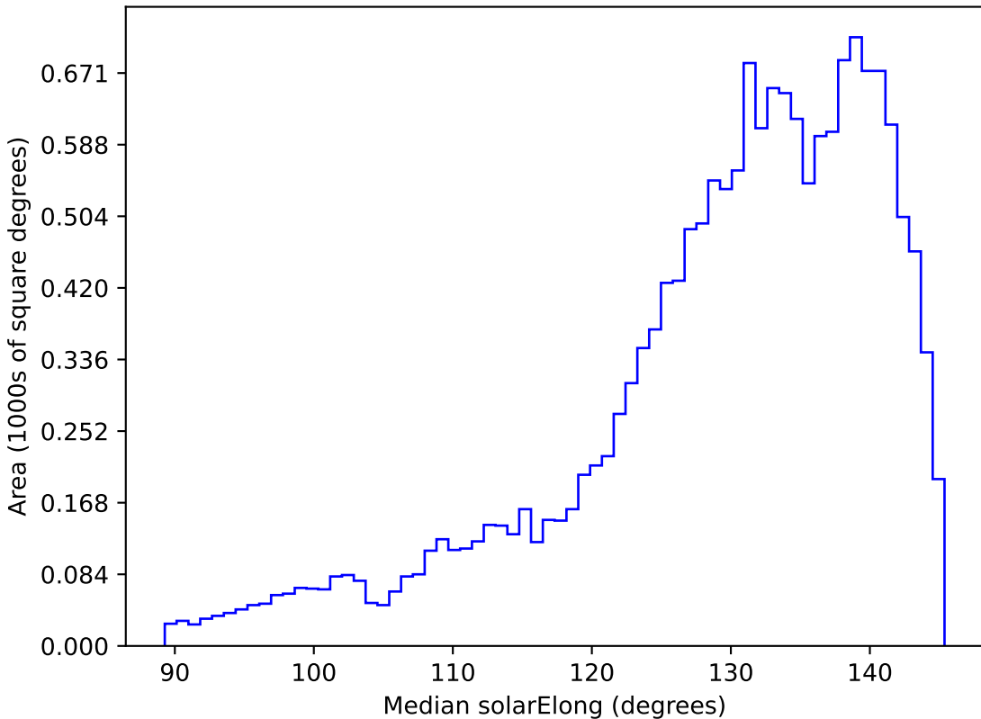
roman_v3.3_10yrs WFD all bands: Median solarElong
