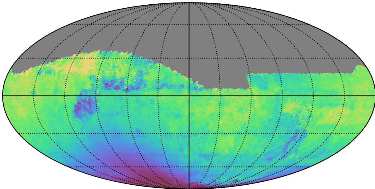
roman_v3.3_10yrs All sky z band: Median solarElong
