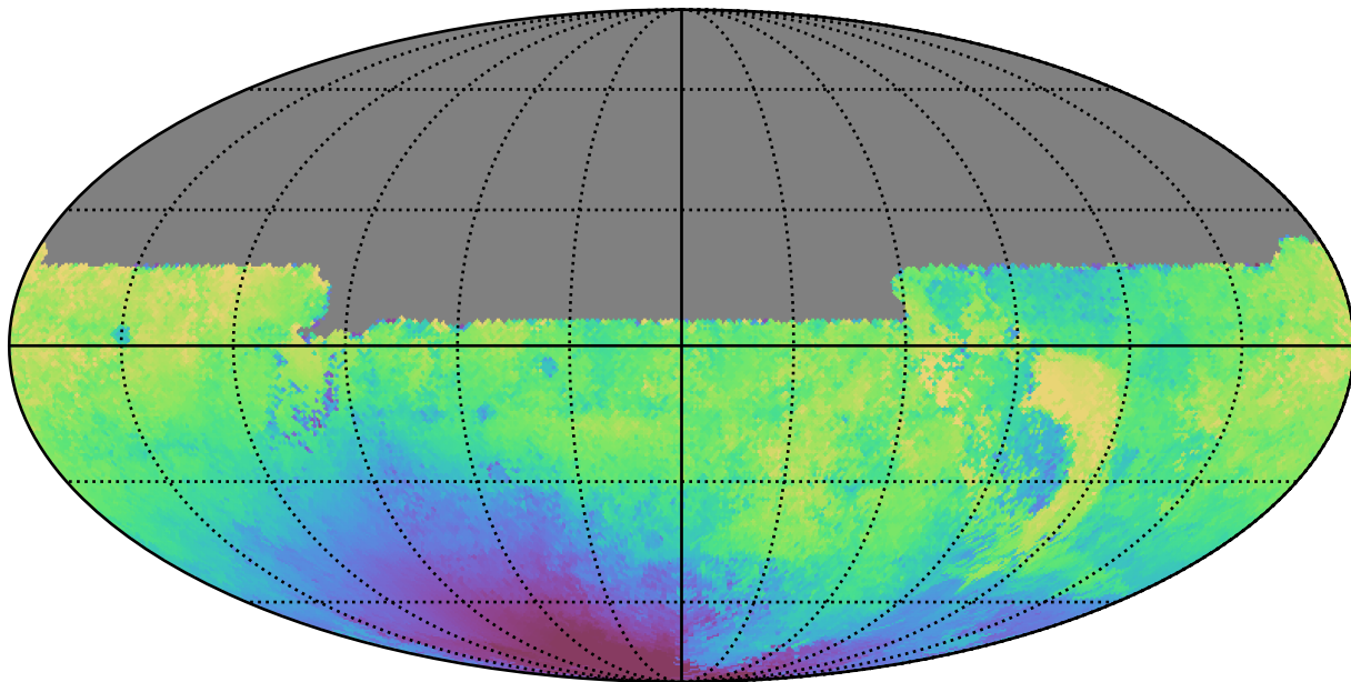
roman_v3.3_10yrs All sky u band: Median solarElong
