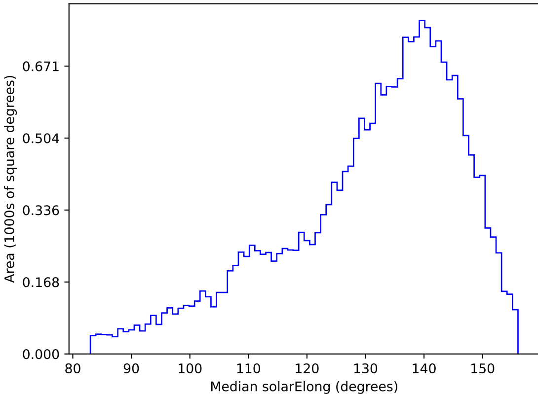
roman_v3.3_10yrs All sky u band: Median solarElong
