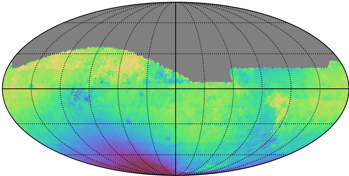
roman_v3.3_10yrs All sky r band: Median solarElong
