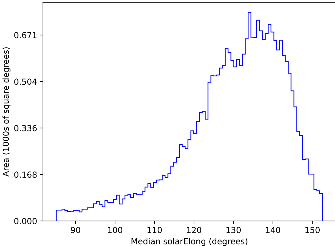
roman_v3.3_10yrs All sky r band: Median solarElong
