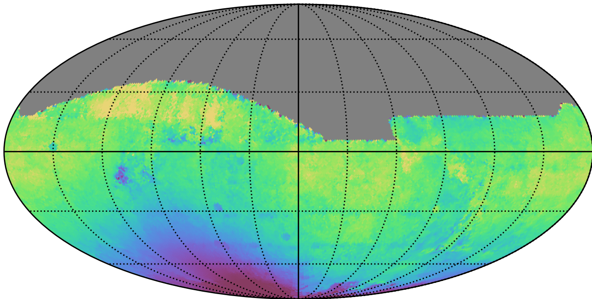
roman_v3.3_10yrs All sky i band: Median solarElong
