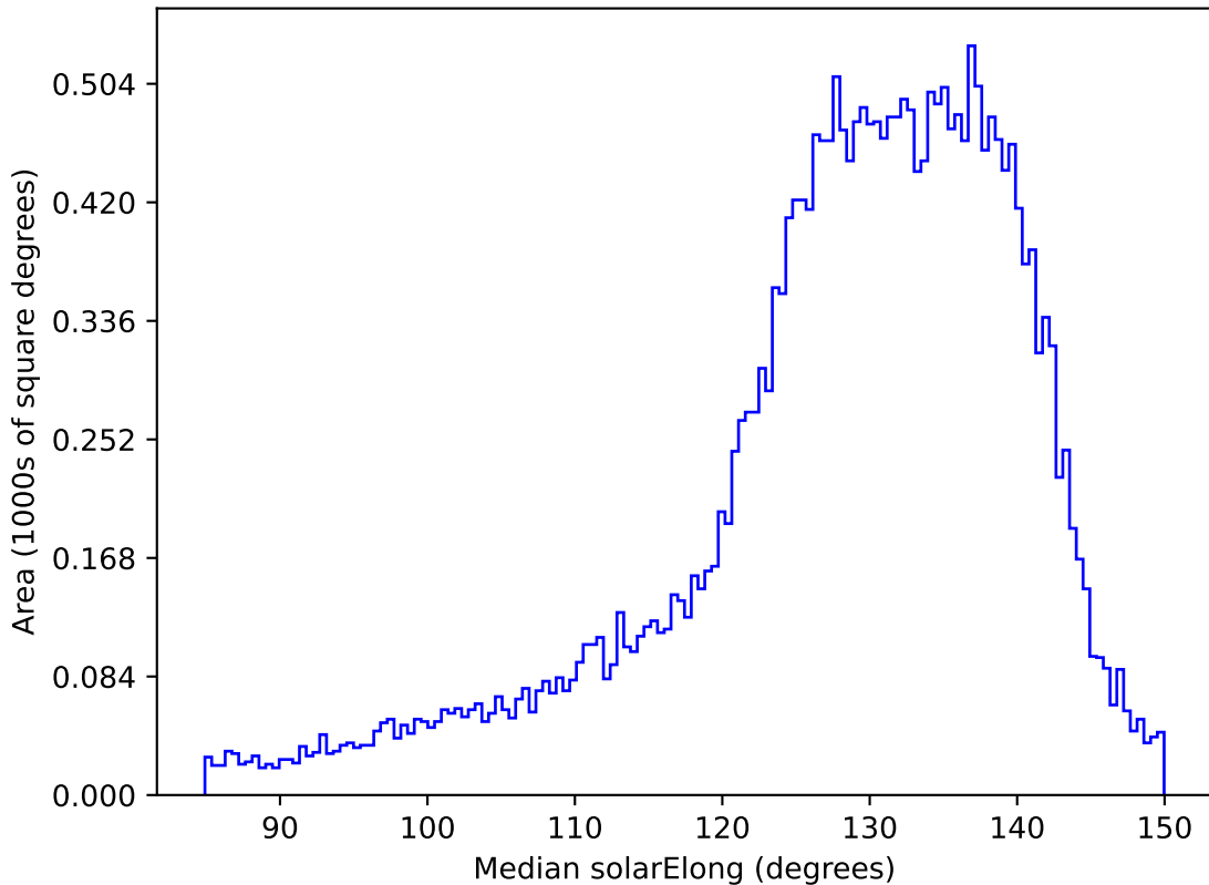
roman_v3.3_10yrs All sky i band: Median solarElong
