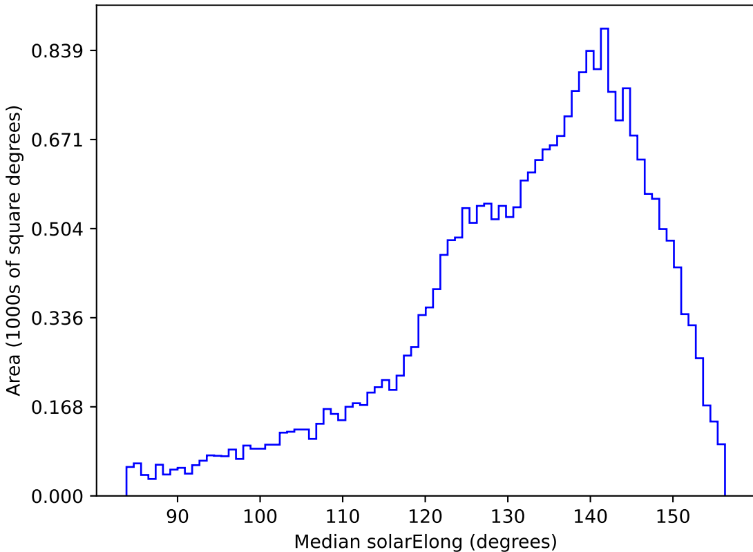
roman_v3.3_10yrs All sky g band: Median solarElong
