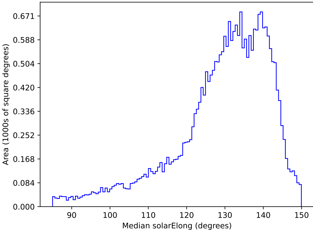
roman_v3.3_10yrs All sky all bands: Median solarElong
