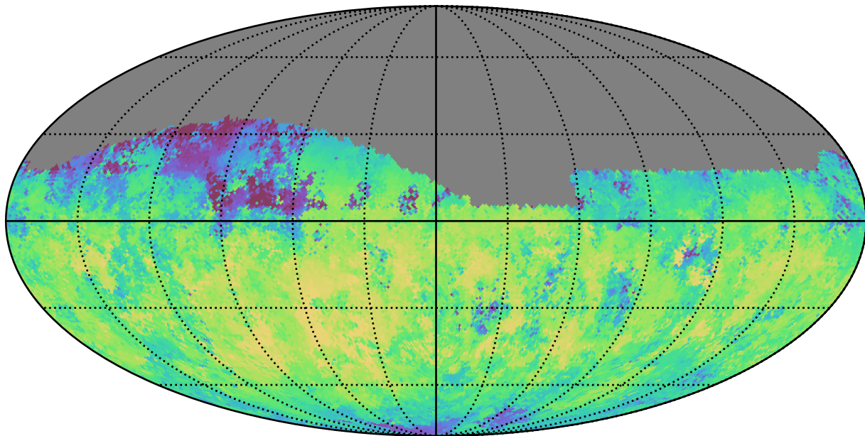
roman_v3.3_10yrs Yr 1 z band: Median skyBrightness
