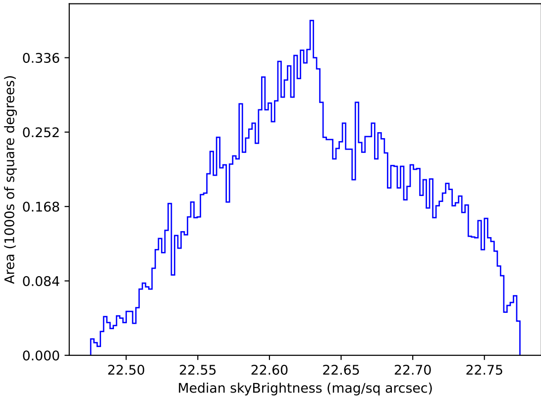
roman_v3.3_10yrs Yr 1 u band: Median skyBrightness
