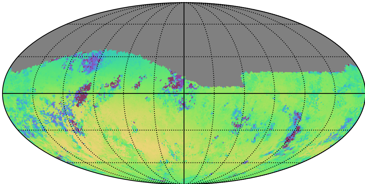
roman_v3.3_10yrs Yr 1 r band: Median skyBrightness
