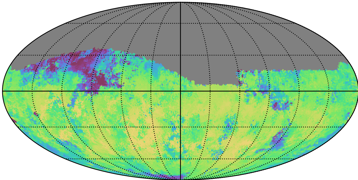
roman_v3.3_10yrs Yr 1 i band: Median skyBrightness
