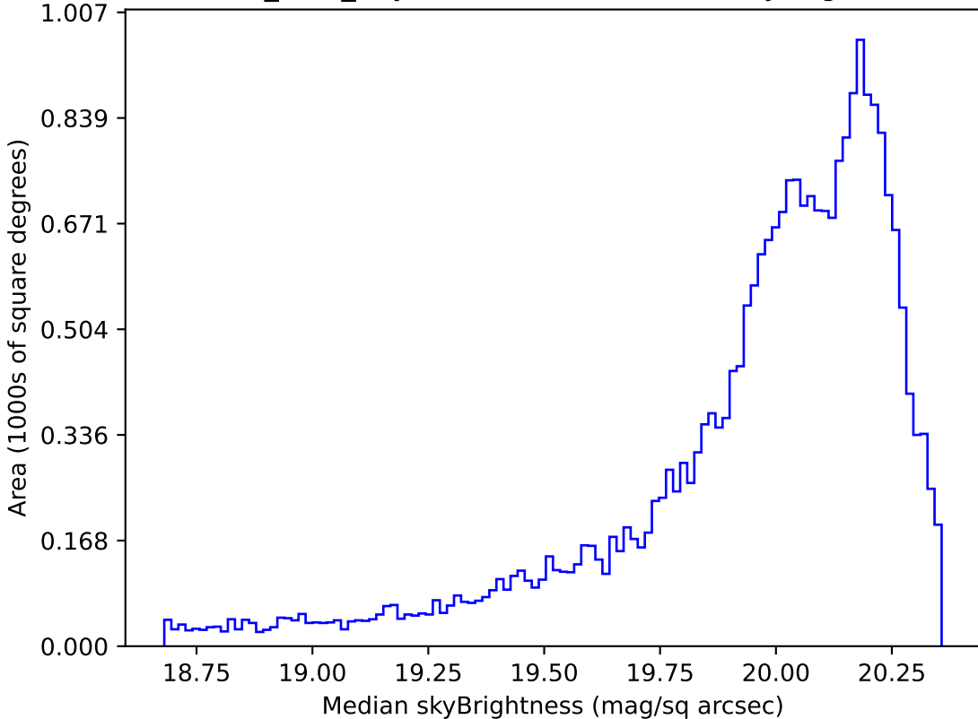
roman_v3.3_10yrs Yr 1 i band: Median skyBrightness
