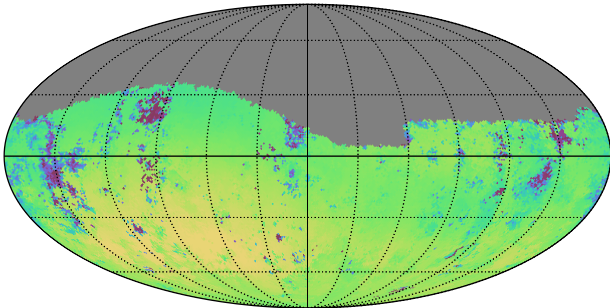
roman_v3.3_10yrs Yr 1 g band: Median skyBrightness
