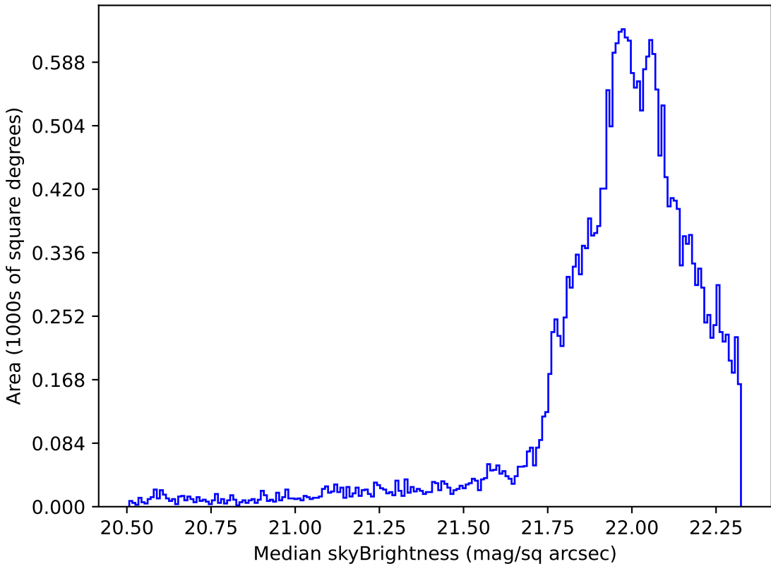
roman_v3.3_10yrs Yr 1 g band: Median skyBrightness
