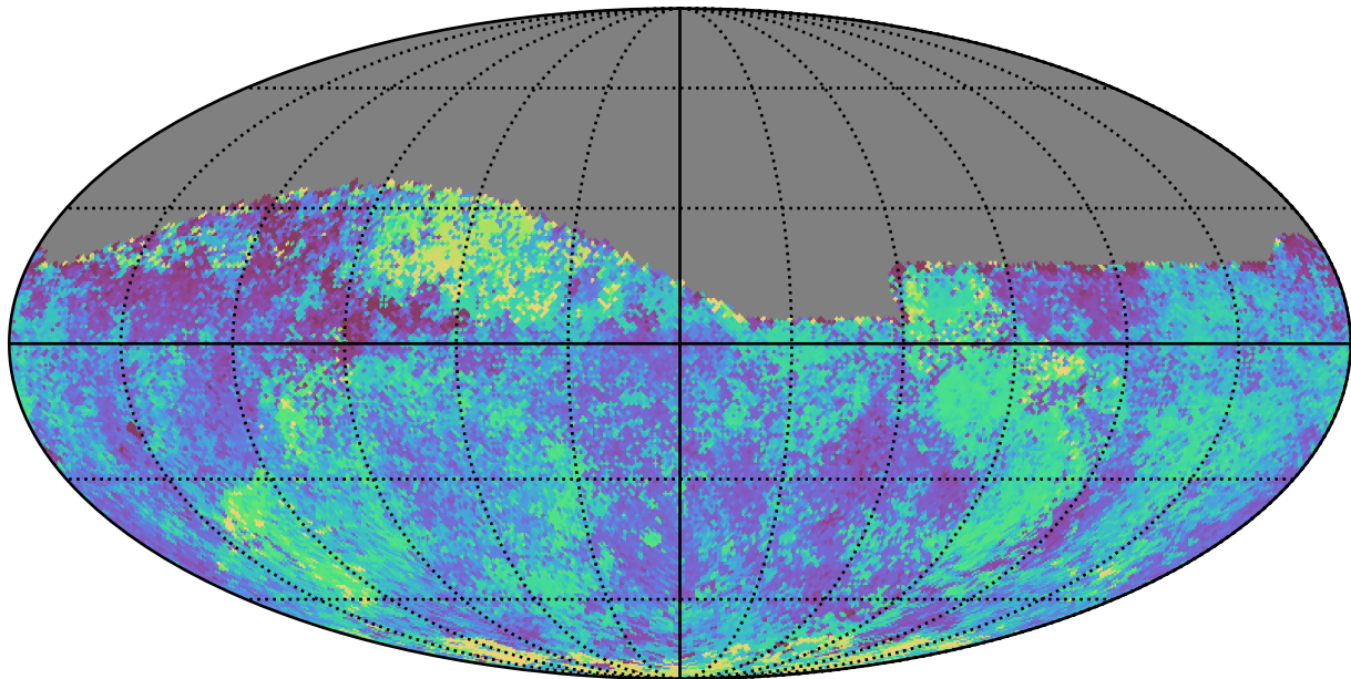
roman_v3.3_10yrs Yr 1 all bands: Median skyBrightness
