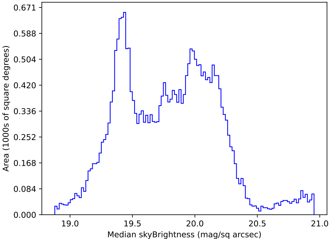
roman_v3.3_10yrs Yr 1 all bands: Median skyBrightness
