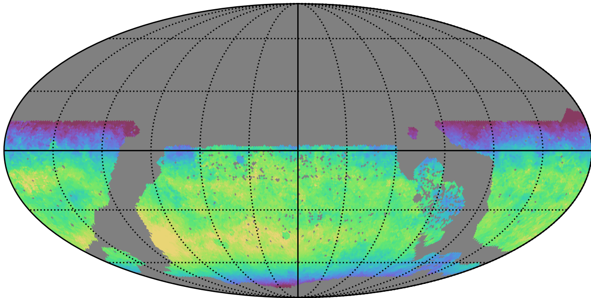
roman_v3.3_10yrs WFD y band: Median skyBrightness
