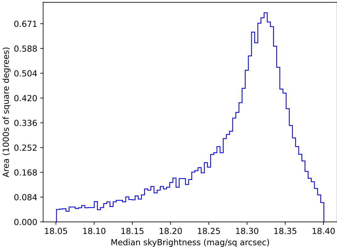
roman_v3.3_10yrs WFD y band: Median skyBrightness
